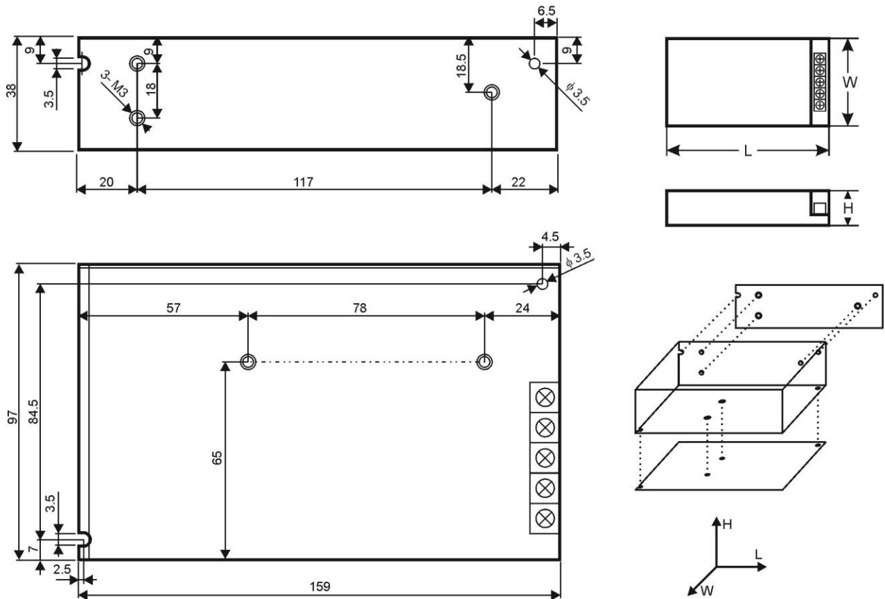
Fig.2. Dimensions of power supply.
