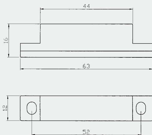
MAGNET
