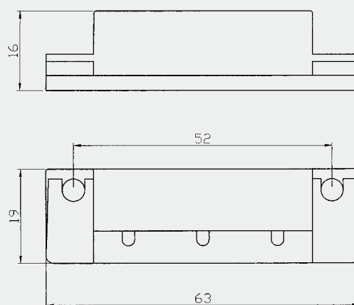
SWITCH
