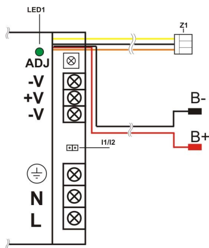
Fig 1. Description of terminals.
